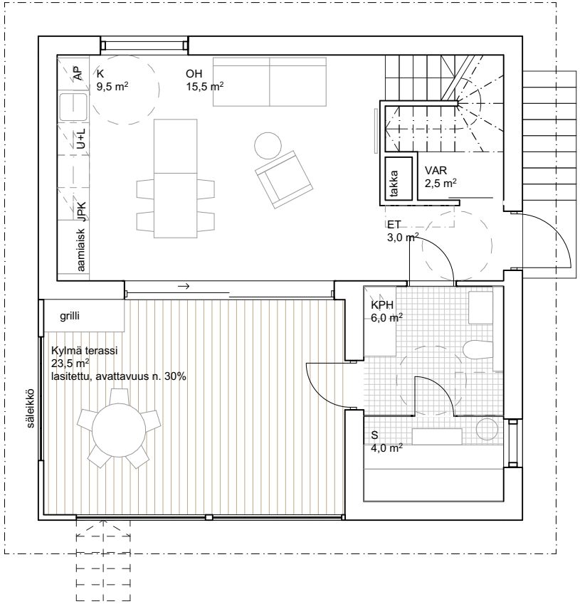
1.krs
